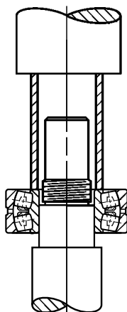
Figure 2: Arbor Press Method
