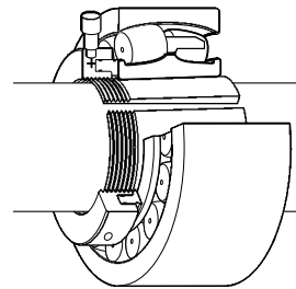
Hydraulic nut used to mount the bearing on a pull type sleeve.
